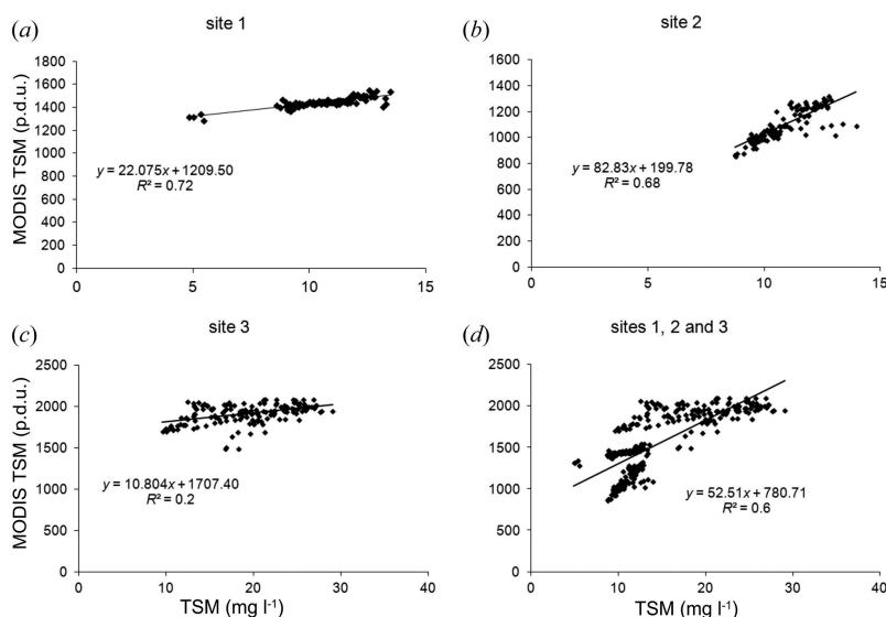
Figure 4. Correlations of TSM concentrations measured by UFL at different sites (a–c) and at all study sites (d) with MODIS satellite data, band 1, 250 m \times 250 m resolution. Lidar data is averaged within each MODIS pixel (p.d.u. – procedure defined units).
