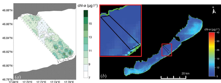
Figure 10. Spatial distribution of chl- a concentrations measured by UFL (a) together with MODIS, the ratio of band 3 to band 4, 500 m \times 500 m resolution (b) in Szemes region (site 2).
